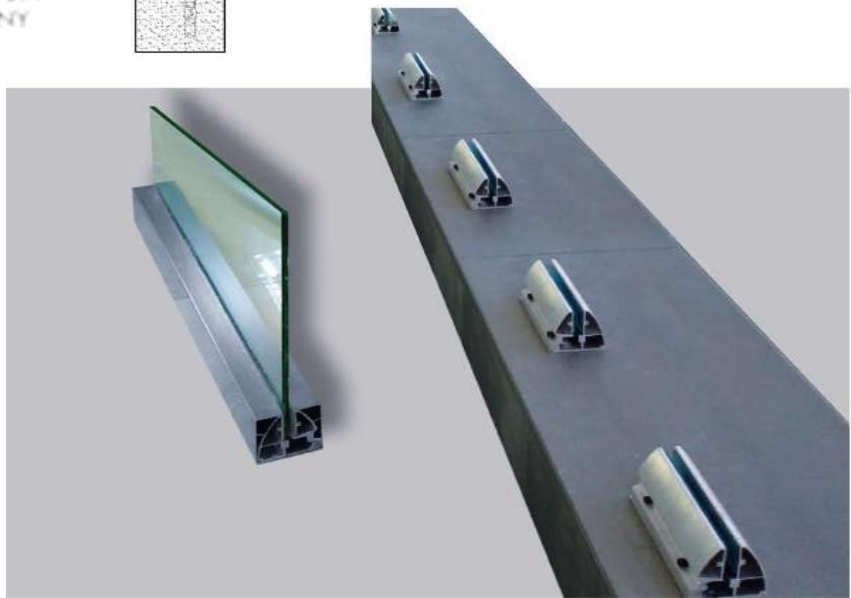
PESPA 006 HORIZONTAL GLASS WALL
